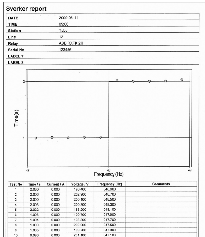
Frequency relay test report
